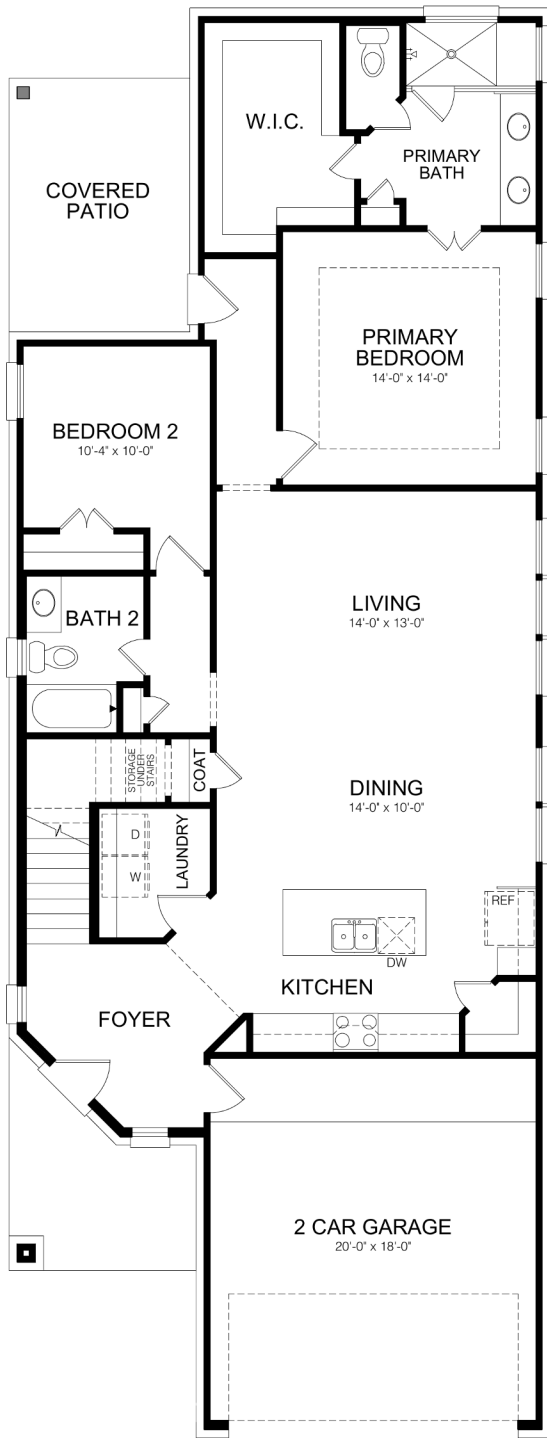
MAIN FLOOR PLAN ELEVATION A
