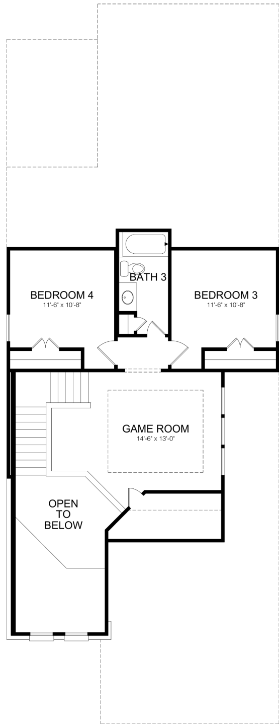
SECOND FLOOR PLAN ELEVATION A
